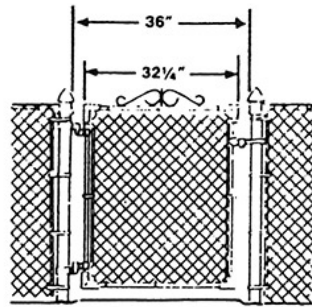
3' WALK GATE
